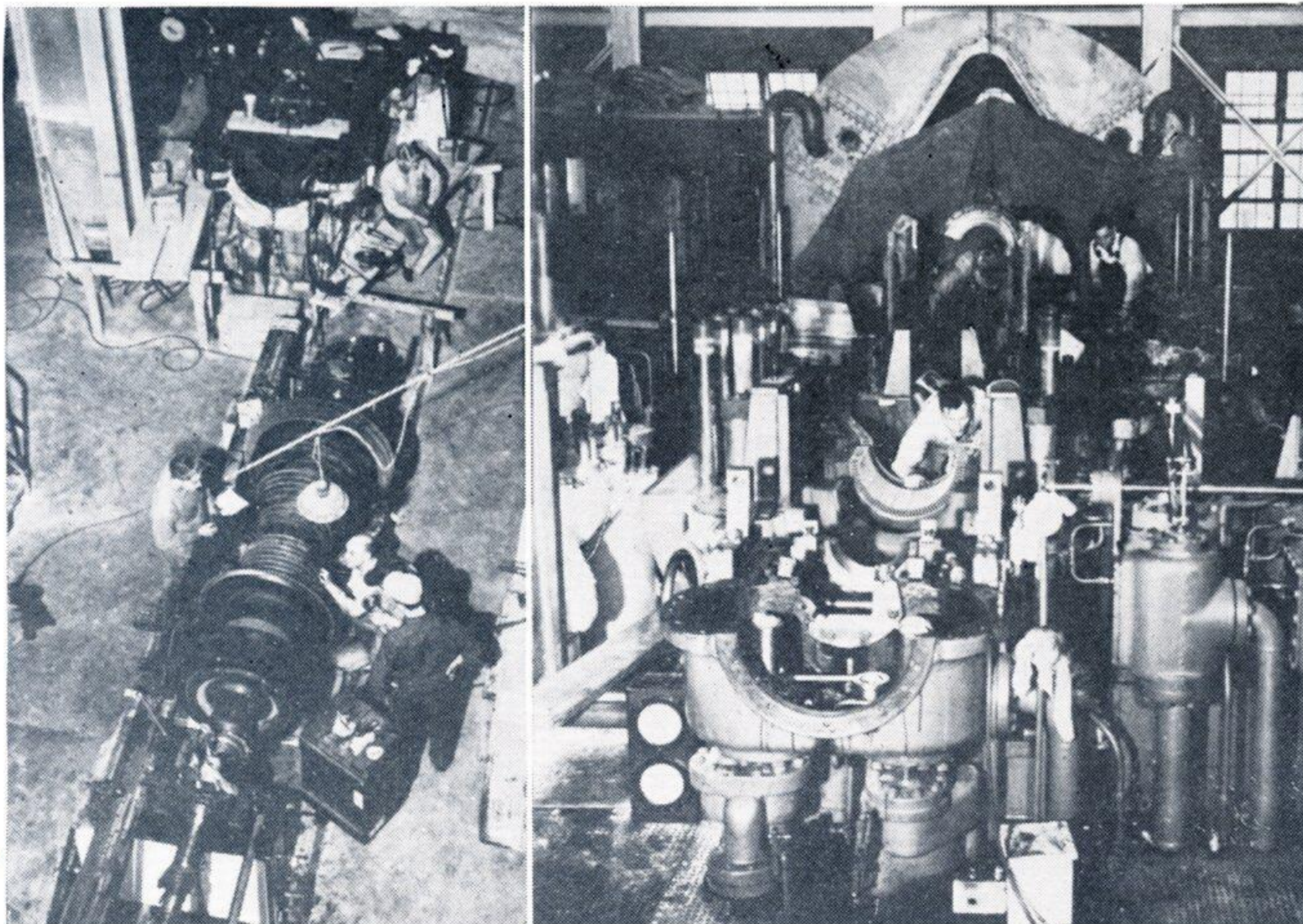
A ROW OF BLADING on Riverside's high pressure spindle is being replaced in the picture on the left. Special frames for holding the rotor were made on the ground floor of the plant building and other special equipment had to be devised by plant workmen especially for this job. At right, measurements are being made for replacing blading on the high pressure cylinder of the turbine.
