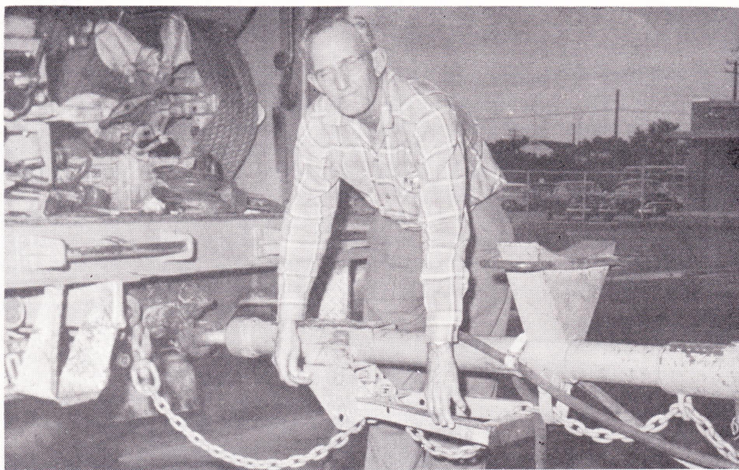
A. D. "Happy" McMillian displays the trailer tongue rest that he devised as a safety measure. A pin locks the rest either up or down. The device allows hitching and unhitching the heavy service trailers with less strain on the men.
