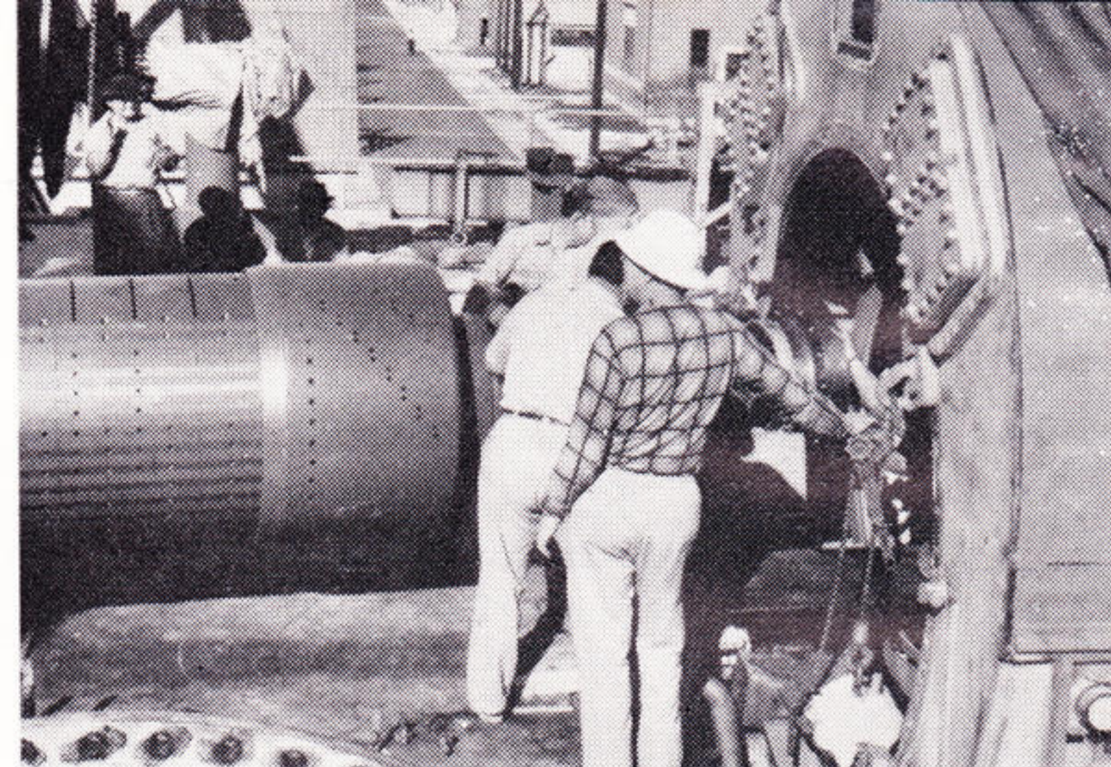
The crew is removing the rotor, the last step in the tear-down. Approximately ten working days were required to reach this point in the overhaul.
